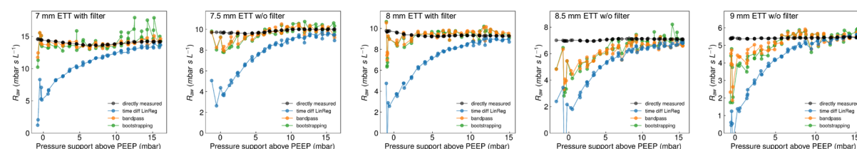
Fig. 3: Performance of the method at different pressure-support levels. Directly measured (black) and estimated (colored) tube resistance values at a flow of 1 L/s are shown as a function of pressure-support level during patient-triggered inspiratory pressure support, for endotracheal tubes of different diameters with or without a bacterial filter. Tube resistance was estimated with three different methods. With increasing pressure support, the estimated values approached the directly measured
