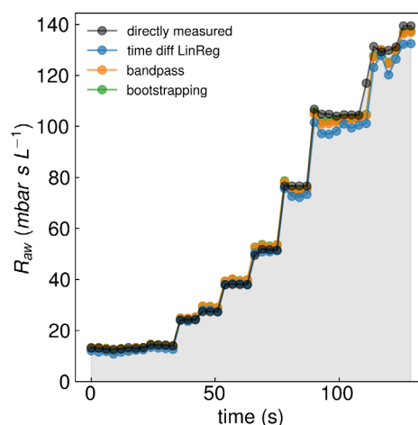
Fig. 4: Continuous detection of tube obstruction. Measured and estimated tube resistance at a flow of 1 L/s during progressive obstruction of a 7 mm endotracheal tube by a 5 mm bronchoscope. Jumps in the data indicate time points at which the bronchoscope was advanced rapidly by several centimeters. Each symbol represents data from one breath.
