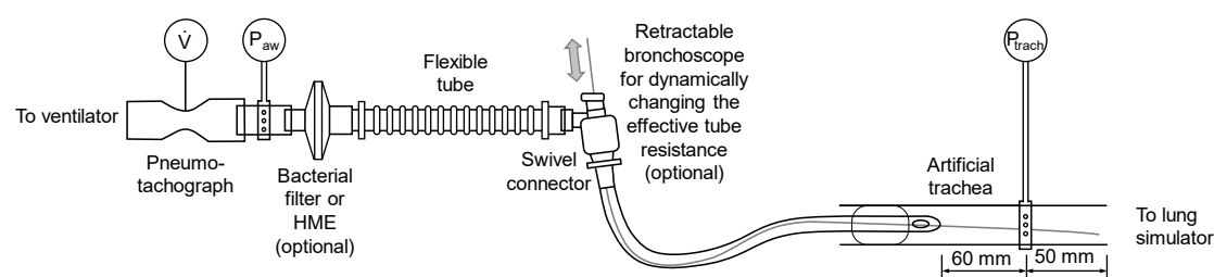
Fig. 1: Experimental setup for measuring tube resistance. The endotracheal tube was inserted into an artificial trachea. To simulate an obstruction, a bronchoscope was advanced through the tube beyond the tracheal pressure measurement site. Tracheal pressure was measured only to validate the resistance values estimated from airway pressure and flow fluctuations.
