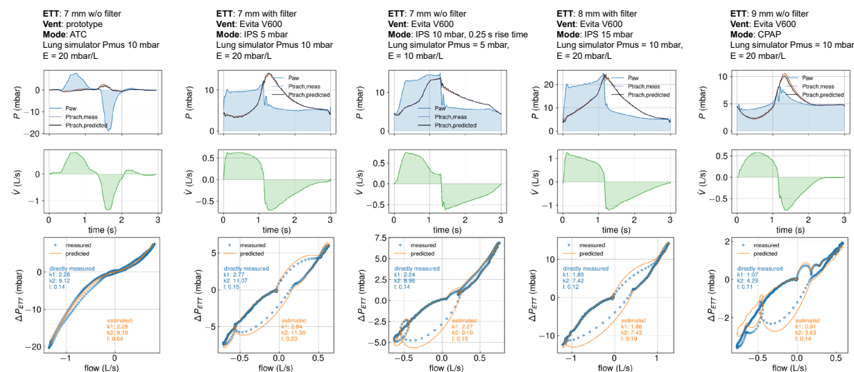
Fig. 2: Performance of the method under different conditions. Each panel shows measured airway pressure, measured and estimated tracheal pressure (top), flow (middle), and measured and estimated pressure drop across the endotracheal tube, including the bacterial filter if present (bottom), during a single breath. The predicted pressure drop, \Delta P_{ETT,calc} , was calculated using Eq. 4 from tube resistance and inertance parameters estimated by the band-pass filtering method from that breath. Estimated tracheal pressure was then obtained as P_{trach,predicted} = P_{aw} - \Delta P_{ETT,calc} . Flow was delivered either by a commercial ventilator (Evita V600) or by a prototype ATC ventilator via endotracheal tubes of different sizes, with or without a bacterial filter, as indicated in the figure.
